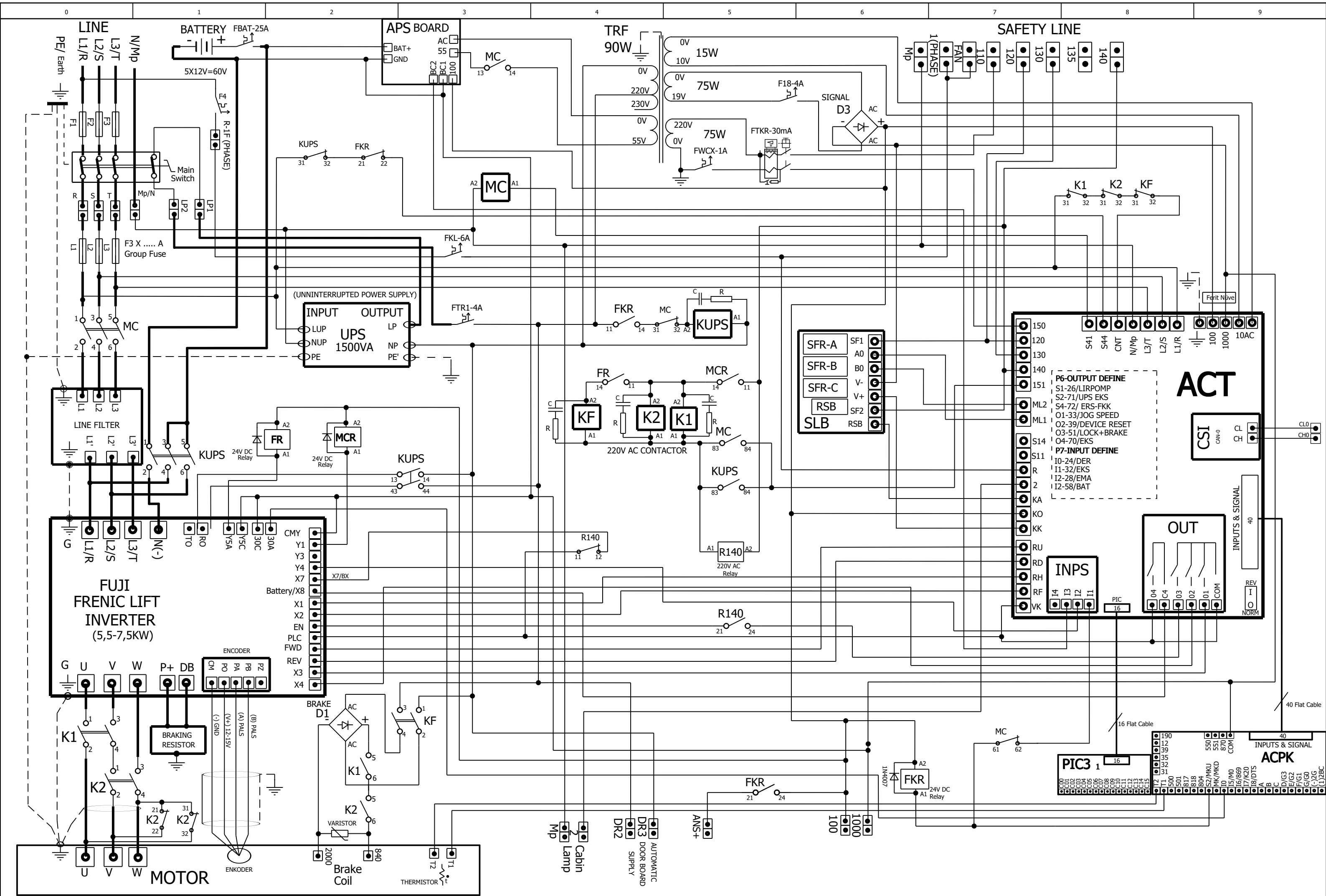
ACT-FRENICLIFT INVERTER BAT+UPS CONNECTIONS DIAGRAM
