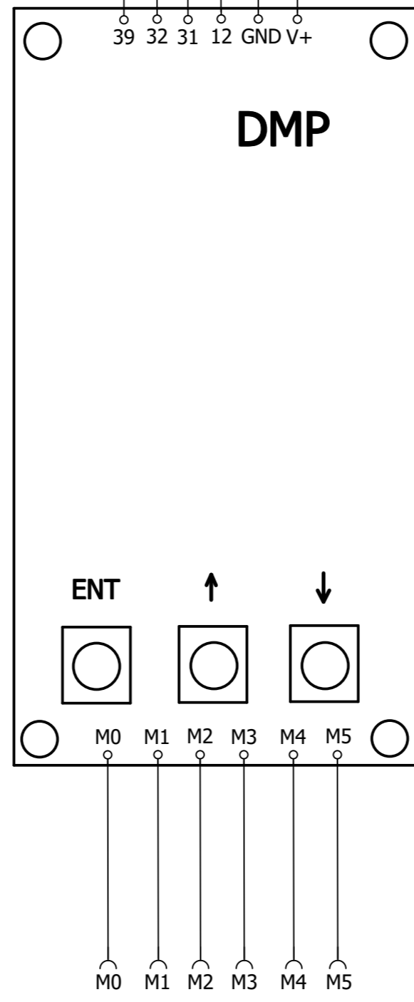
Control Panel GrayCode Outputs
