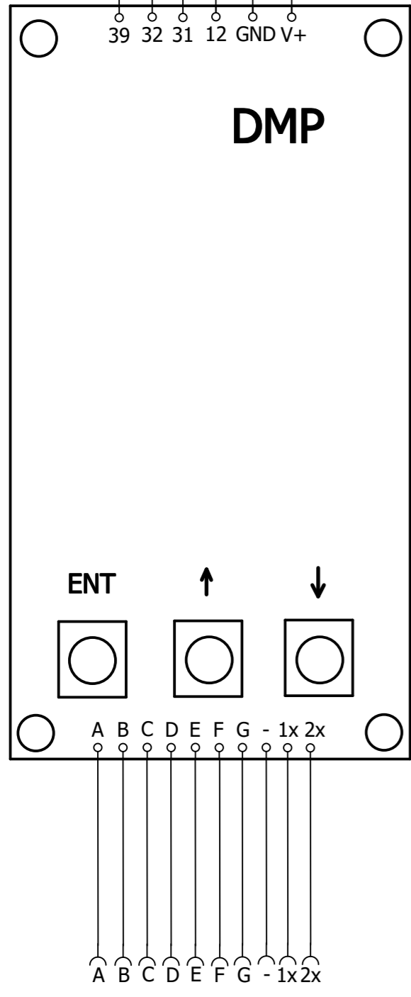
Control Panel Seven Segment Outputs
