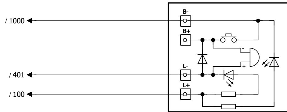
ÇİFT RENK TWO COLOR BUZZERLİ AND BUZZER KAYIT BUTONU CALL BUTTON
