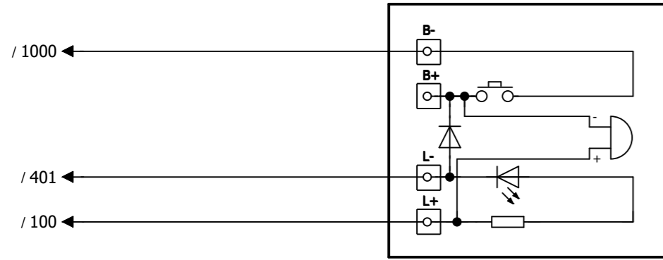
TEK RENK ONE COLOR BUZZERLİ AND BUZZER KAYIT BUTONU CALL BUTTON
